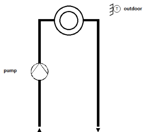
Figure 3-2 Unmixed heating circuit
