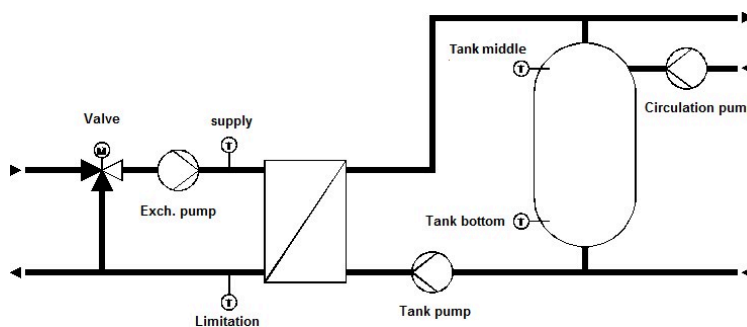
Figure 3-13 Storage tank charging systems with two point controlled tank and PI controlled load supply temperature
