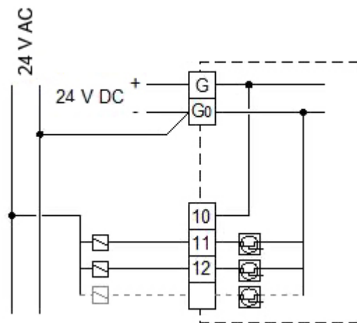
Figure 4-8 24 V DC supply and 24 V AC relays
