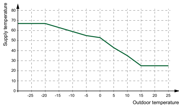
Figure 2-3 8-point curve
