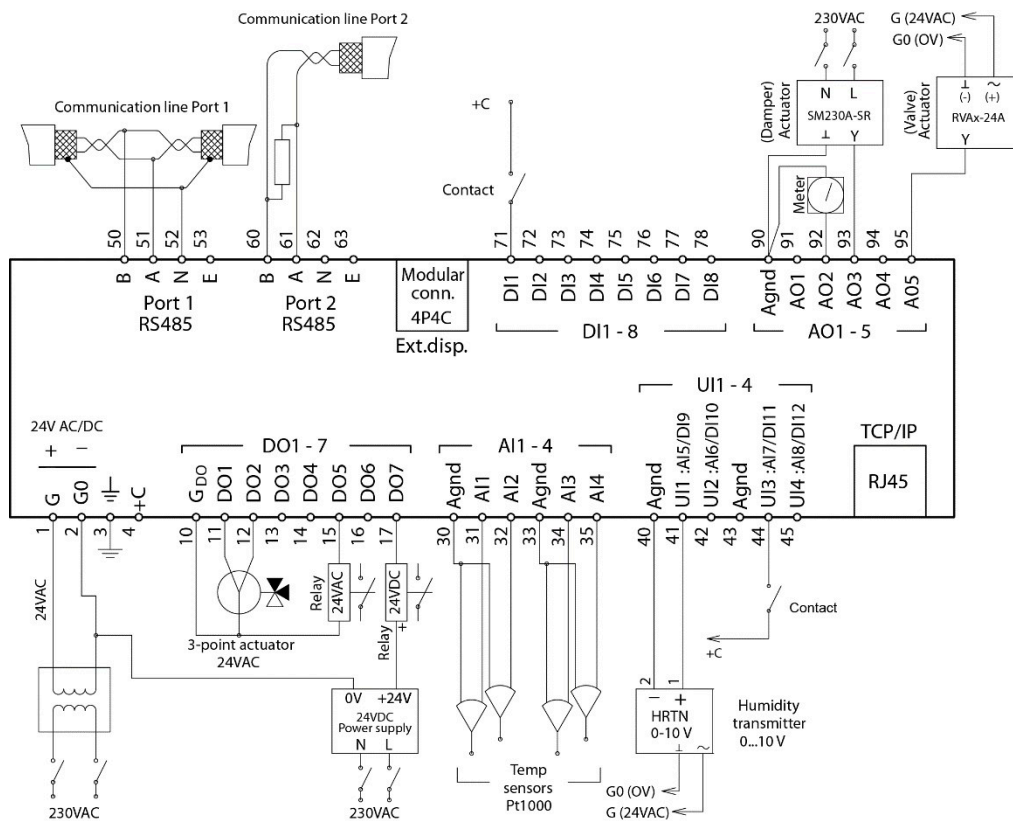
Figure 4-3 Wiring example
