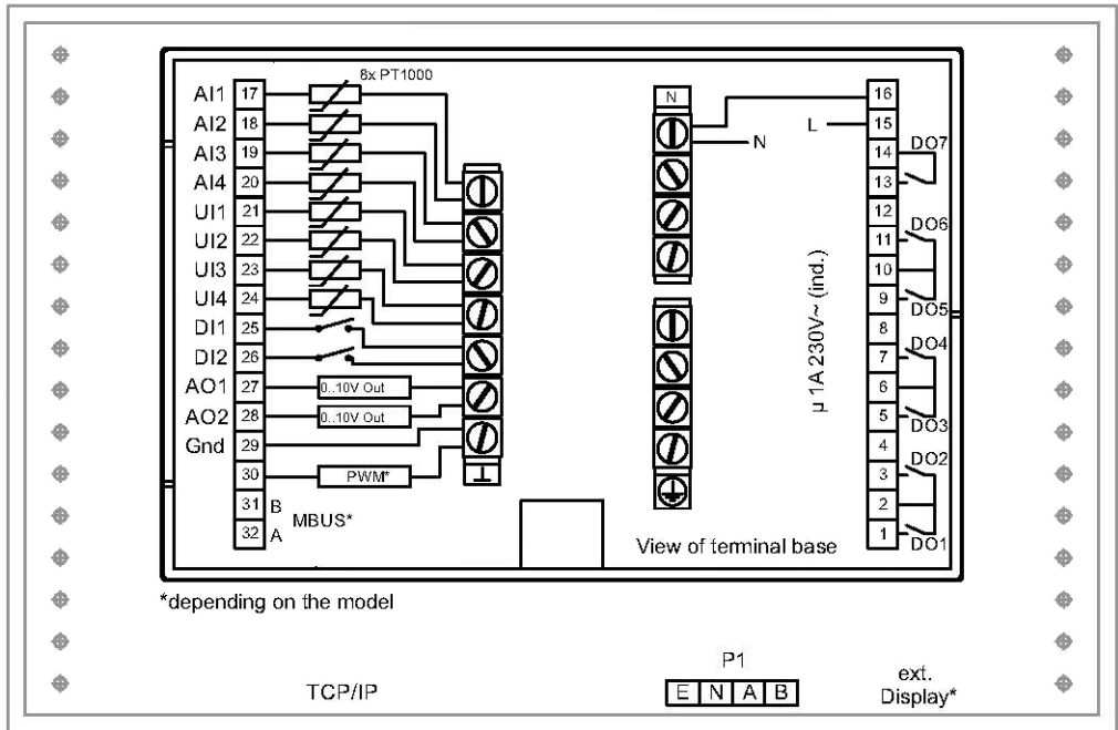
Figure 4-2 Terminal positions 230 V models (Exigo Vido)
