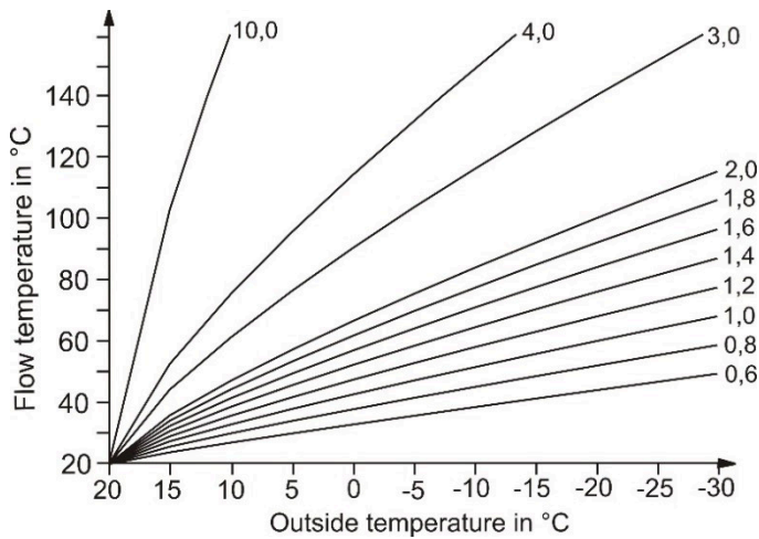
Figure 2-5 DIN curve slope
