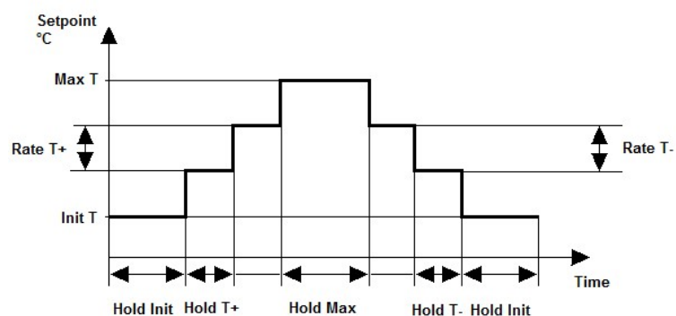
Figure 3-9 Screed drying
