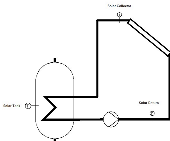
Figure 3-19 Solar circuit
