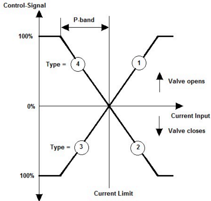
Figure 3-7 Universal limitation
