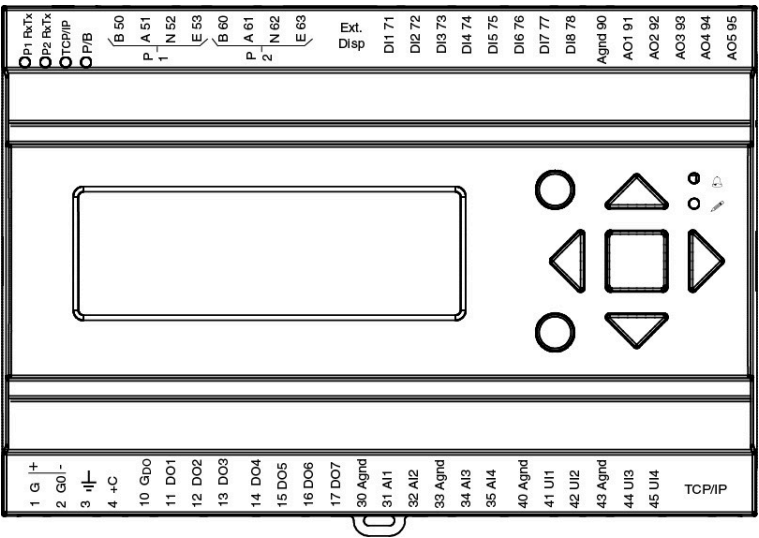
Figure 4-1 Terminal positions 24 V models (Exigo Ardo)
