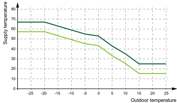
Figure 2-4 8-point curve with displacement
