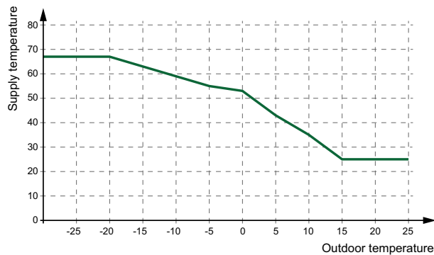
Figure 3-3 8-point curve
